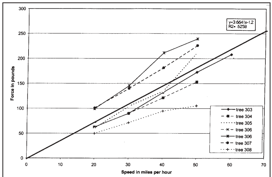
Figure 4. Wind resistance of green ash ( Fraxinus pennsylvanica ) measured at various speeds 24 in. (61 cm) above original grade. Odd-numbered trees were grown within root barriers. Bold line is the regression line for all trees.
